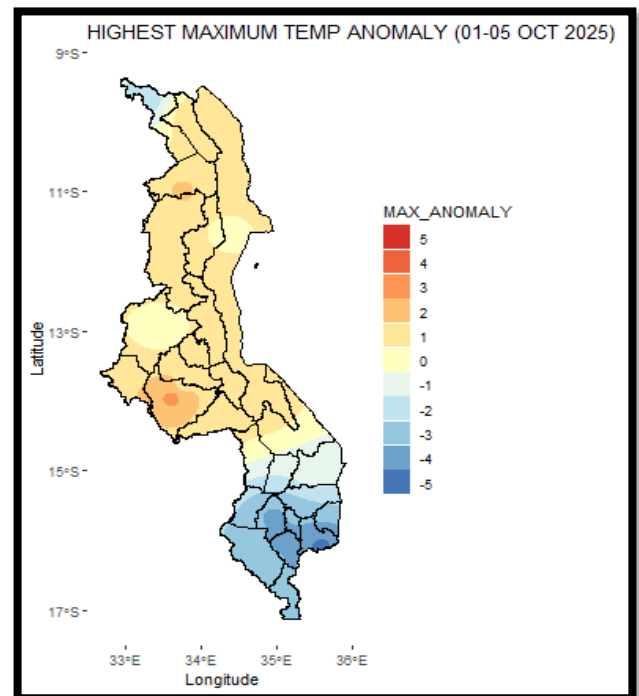
Highest maximum temperature anomalies reported and compared to October historical temperature.
