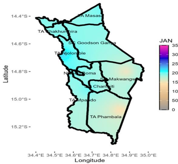
JANUARY 2027 RAINFALL FORECAST
