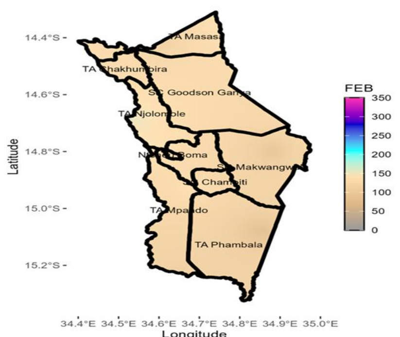
FEBRUARY 2027 RAINFALL FORECAST
