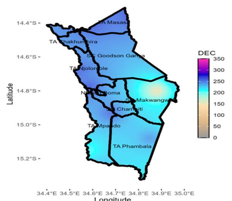
DECEMBER 2026 RAINFALL FORECAST
